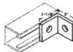
L11 2 Hole Corner Angle
