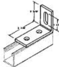
L21 1 Slot - 2 Hole Corner Angle
