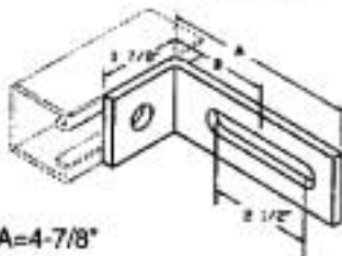
L16, L17 1 Slot - 1 Hole Angle
