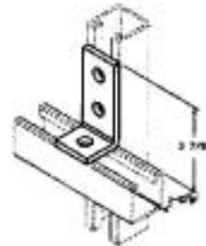
L19 3 Hole Corner Angle
