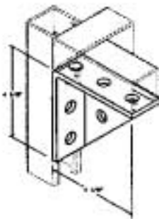
L23 7 Hole Corner Angle
