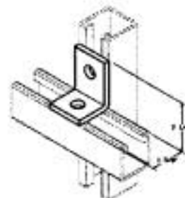
L10 2 Hole Corner Angle
