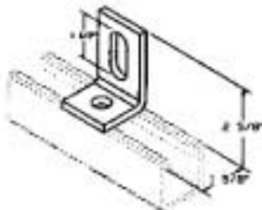
L15 1 Slot - 1 Hole Angle
